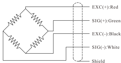
Wiring Diagram
