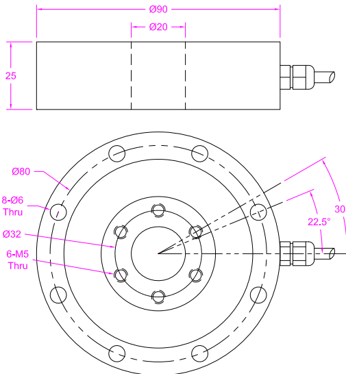
Model:THE Capacity:10/20/30/40/50NM
