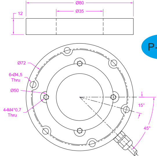
Model:THF Capacity:10/20/30/50NM
