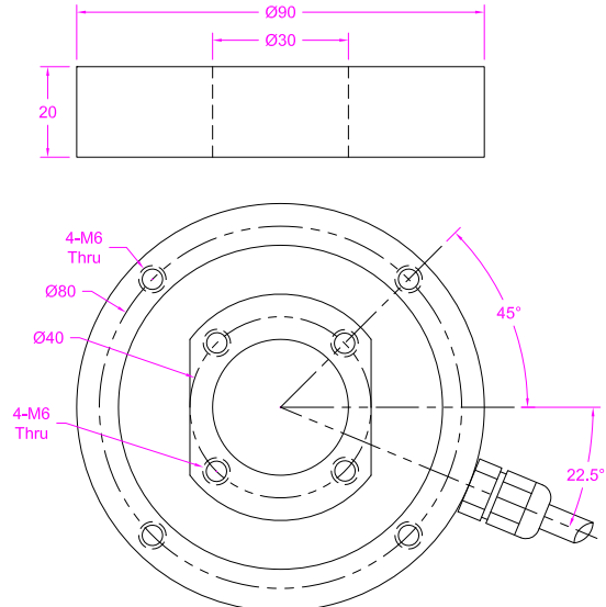
Model:THF Capacity:10/20/30/50NM
