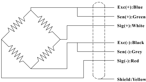
Wiring Diagram @ Tension
