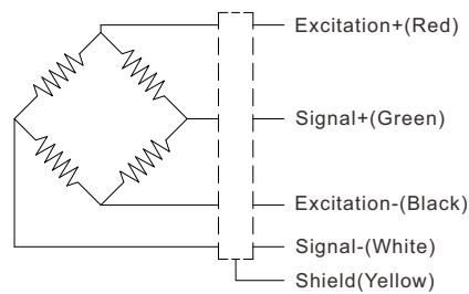
Wiring Code (Same for Fx/Fy/Fz axis)
